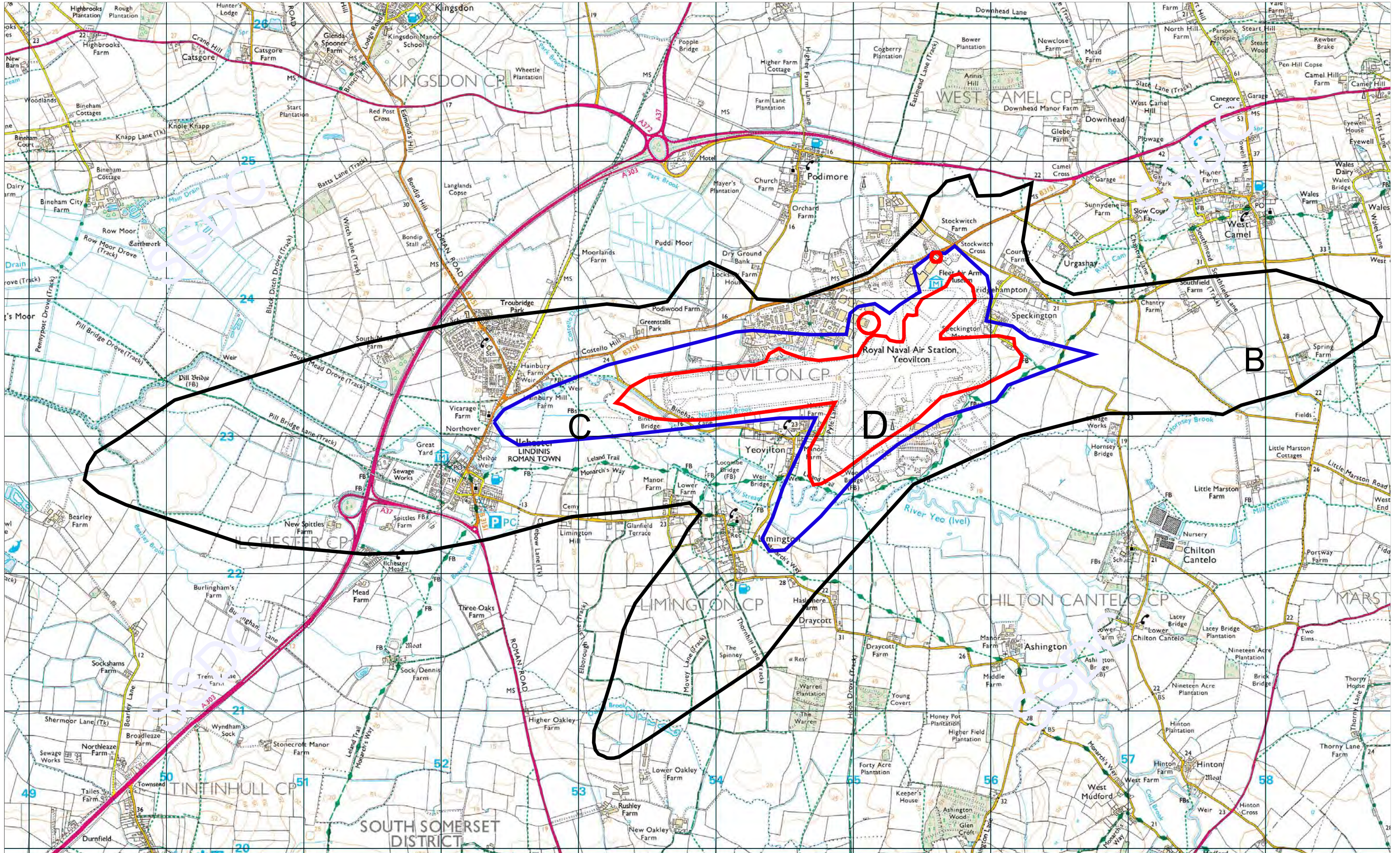
Noise Exposure categories for RNAS Yeovilton - Appendix 4A (July 2010)
